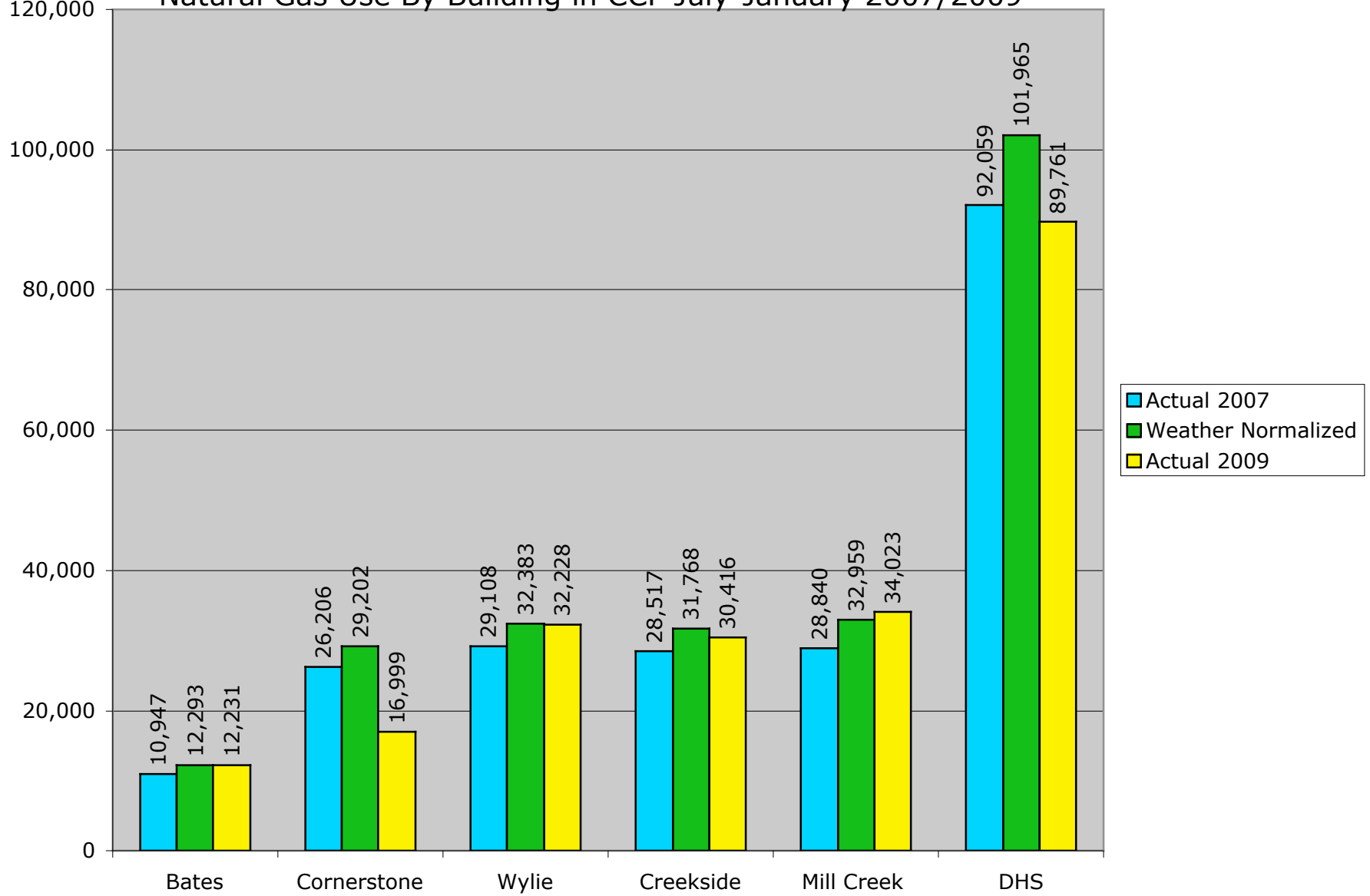
Natural Gas Use By Building in CCF July-January 2007/2009
